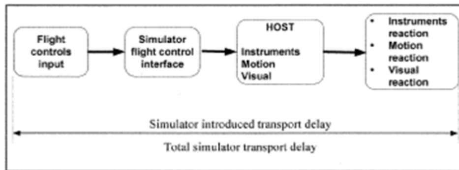
Figura 1-IIC Transport delay for simulation of classic non-computer controlled aircraft
