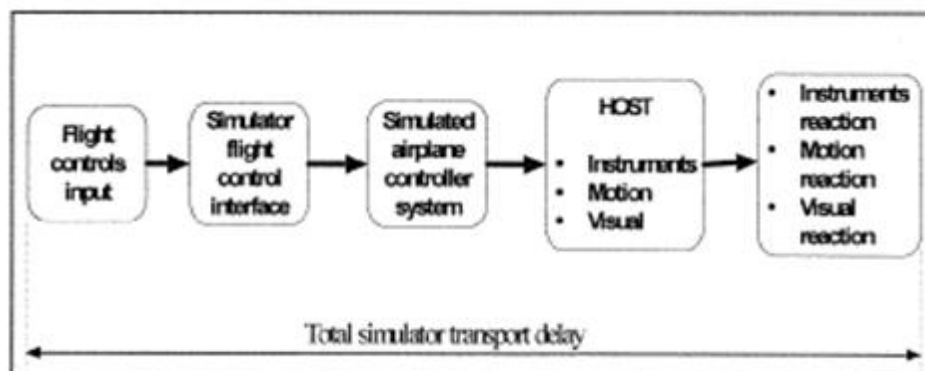
Figura 1-IIE Transport delay for simulation of computer controlled aircraft using software emulation of airplane boxes
