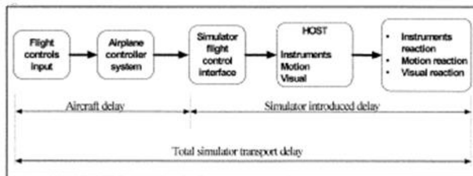
Figura 1-IID Transport delay for simulation of computer controlled aircraft using real airplane black
