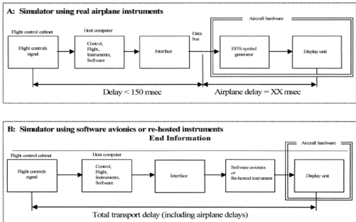
Figuras 1-IIF(A) y 1-IIF(B) – Transport delay for simulation of airplane using real or re-hosted instrument drivers
